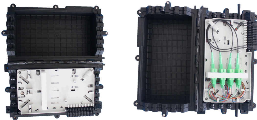
HTSC-145 product picture
